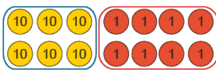
Figure 27: place-value counters showing 34 \times 2
