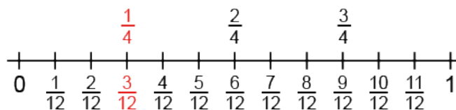
Figure 38: number line showing that \frac{1}{4} and \frac{3}{12} are equivalent
