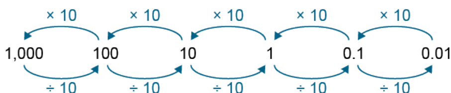
Figure 23: multiplicative relationships between powers of 10: 10 times the size and one-tenth times the size
