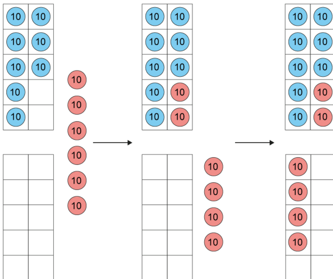
Figure 14: tens frames with 10-value counters showing 80 + 60 = 140
