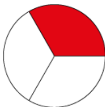
Figure 29: a circle divided into 3 equal parts, with one part shaded
